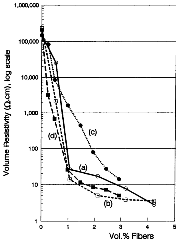
Figure 13 Variation of the volume electrical resistivity with carbon fiber volume fraction. (a) Without sand, with methylcellulose, without silica fume. (b) Without sand, with methylcellulose, with silica fume. (c) With sand, with methylcellulose, without silica fume. (d) With sand, with methylcellulose, with silica fume.
