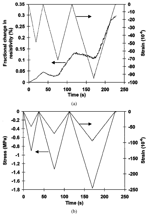
Figure 6 Variation of the fractional change in electrical resistivity with time (a), of the stress with time (b), and of the strain (negative for compressive strain) with time (a,b) during dynamic compressive loading at increasing stress amplitudes within the elastic regime for silica-fume cement paste at 28 days of curing.
