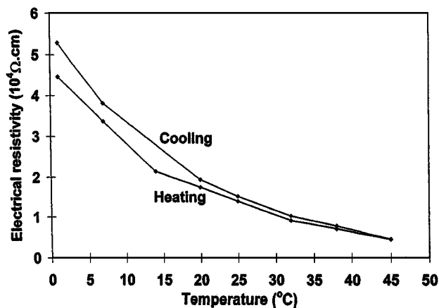
Figure 10 Plot of volume electrical resistivity vs. temperature during heating and cooling for carbon-fiber silica-fume cement paste.
