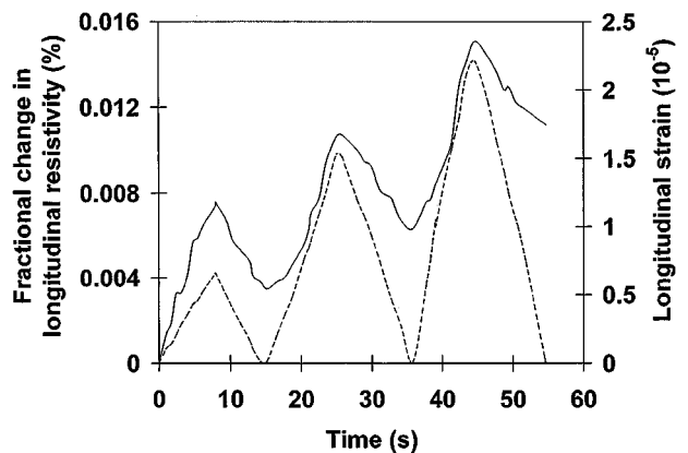
Figure 4 Variation of the fractional change in longitudinal electrical resistivity with time (solid curve) and of the strain with time (dashed curve) during dynamic uniaxial tensile loading at increasing stress amplitudes within the elastic regime for silica-fume cement paste.
