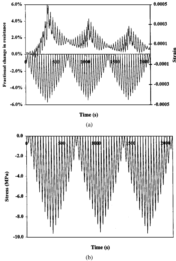
Figure 7 Fractional change in resistance (upper curve in (a)), strain (lower curve in (a)) and stress (b) during repeated compressive loading at increasing and decreasing stress amplitudes, the highest of which was 60% of the compressive strength, for carbon fiber concrete at 28 days of curing.
