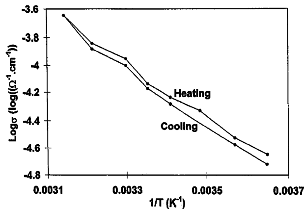
Figure 11 Arrhenius plot of log electrical conductivity vs. reciprocal absolute temperature for carbon-fiber silica-fume cement paste.
