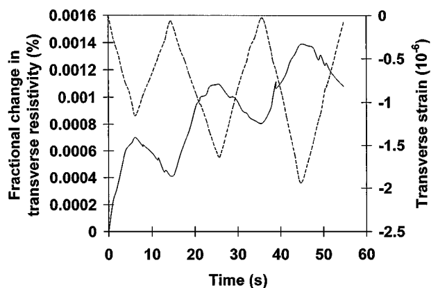
Figure 5 Variation of the fractional change in transverse electrical resistivity with time (solid curve) and of the strain with time (dashed curve) during dynamic uniaxial tensile loading at increasing stress amplitudes within the elastic regime for silica-fume cement paste.
